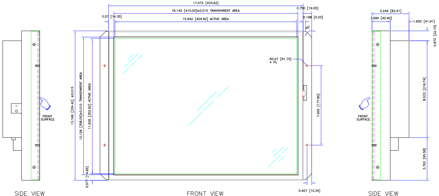
FRONT VIEW
